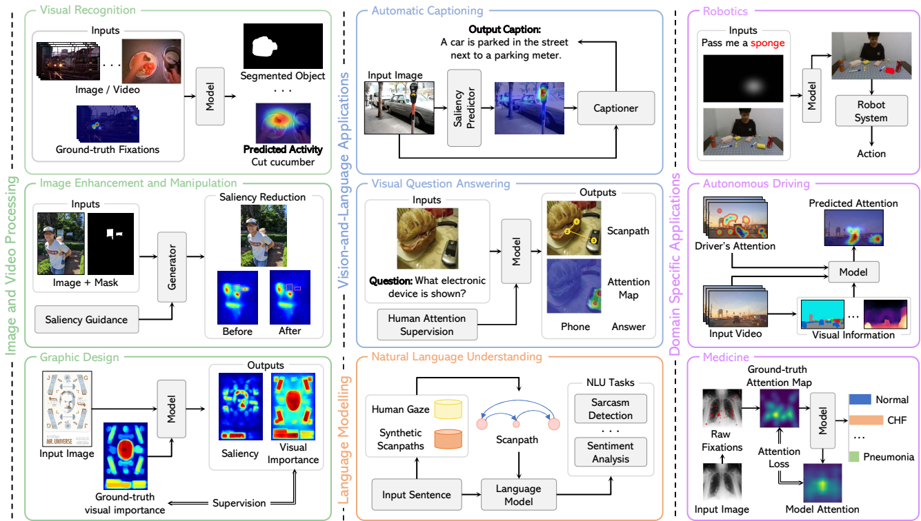
Figure 1: An overview of sample architectures integrating human visual attention with different input and output modalities. Human visual attention has been employed to solve tasks in diverse domains spanning from image and video processing, automatic captioning, visual question answering, and language understanding, as well as robotics, autonomous driving, and medicine.
