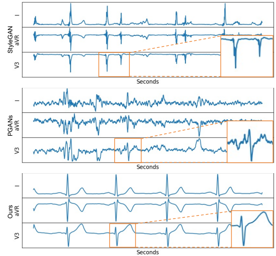
Figure 3: Visualization of ECG generated of STTC (ST/T Change) category by different models. For clarity in comparison, we only use the electrocardiogram of three leads: I, aVR, and V3.
