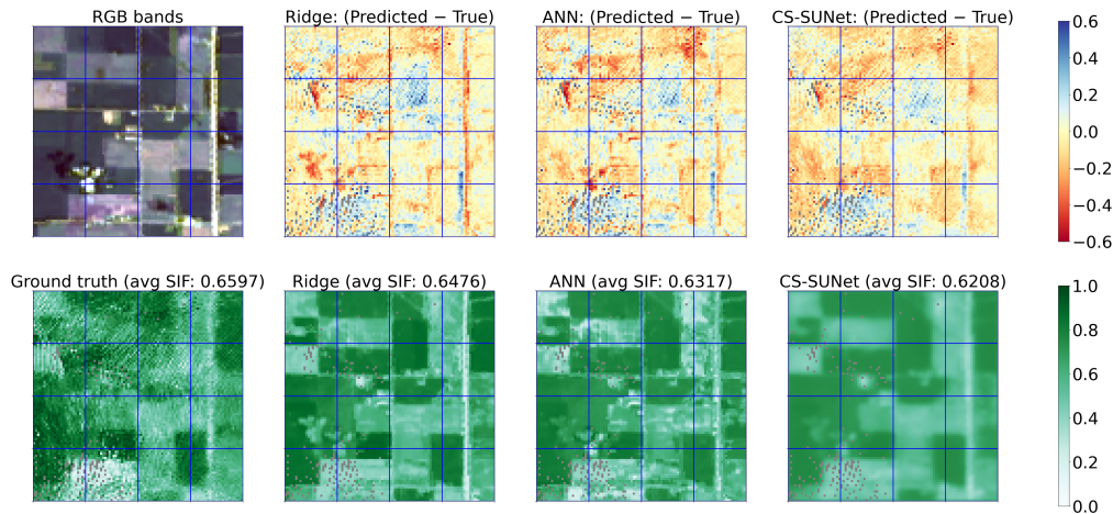
Figure 3: Example result. Top-left: RGB bands, used as input features. Bottom-left: ground-truth CFIS SIF (gray pixels are missing data). Other bottom images: predictions with different methods (CS-SUNet is rightmost). Other top images: error maps (yellow is accurate, blue is over-prediction, red is under-prediction). CS-SUNet is generally more accurate than other methods – for example, there are fewer dark red or blue pixels (which indicate major errors).
