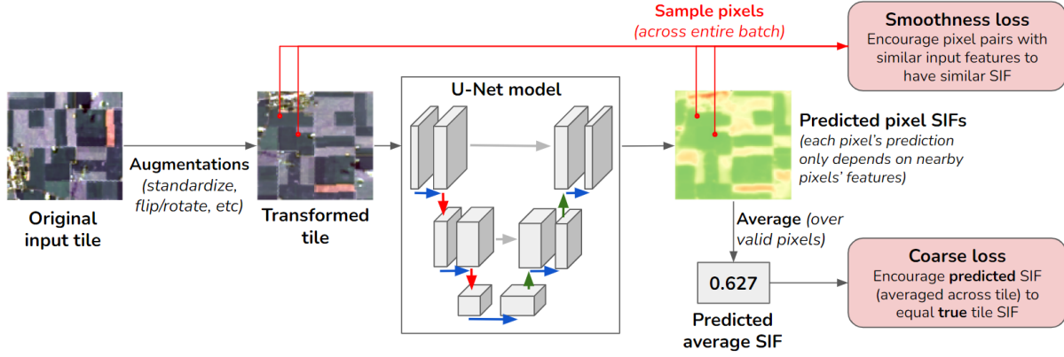
Figure 2: Coarsely-Supervised Smooth U-Net (CS-SUNet). At each iteration, we first apply some augmentations to the original input tile (satellite images, etc). Then we pass it through the U-Net to obtain pixel SIF predictions. Finally, we compute the coarsely-supervised loss and the smoothness regularization loss, and backpropagate to improve the model.
