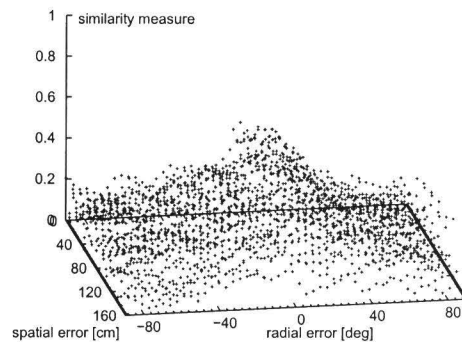
Figure 3: Performance of GLM on real images.
