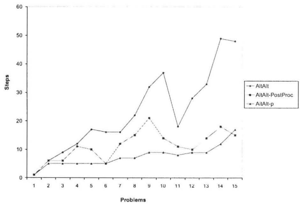
Figure 2: AltAlt and Post-Processing vs AltAlt p
