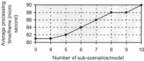
Figure 5. The processing time of the new algorithm is closely linear time in function of the number of sub-scenarios.
