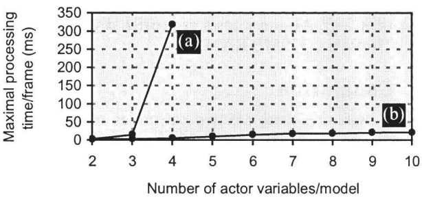
Figure 6. The processing time (a) of the old algorithm and (b) of the new algorithm depend on the number of actor variables of predefined scenario models.
