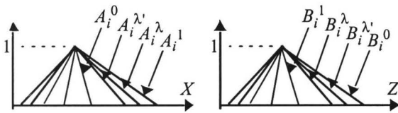
figure 10: Nested fuzzy subsets ( \lambda \geq \lambda' )
