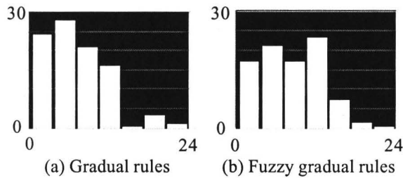
figure 13: Effect of fuzzy gradual rules on the discrimination
