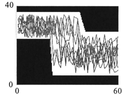
figure 6: Model of class 5 (truncated graph)
