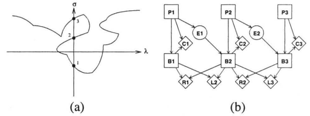
Figure 1: (a) An abstract diagram of the path. The horizontal axis represents \lambda and the vertical axis represents the space of strategy profiles (actually multidimensional). The algorithm starts on the right at \lambda = 1 and follows the dynamical system until \lambda = 0 at point 1, where it has found an equilibrium of the original game. It can continue to trace the path and find the equilibria labeled 2 and 3. (b) Two-stage road building MAID for three agents.
