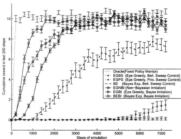
Figure 7: No South results (50 runs)
