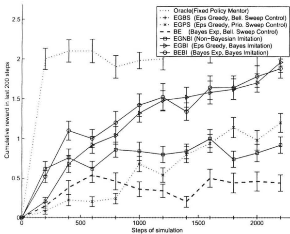
Figure 5: Tutoring domain results (50 runs)
