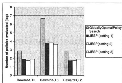
Figure 2: Evaluation Results
