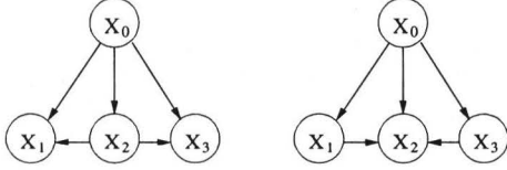
Figure 2: A tree-augmented Naive Bayes (TAN) model satisfying Condition 1 (left); and a network that is not TAN (right). Even though in both cases the class variable X_0 is a moral node, the network on the right does not satisfy Condition 1.
