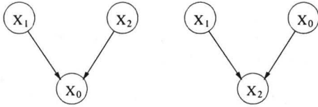
Figure 1: A simple Bayesian network (the class variable is denoted by X_0 ) satisfying Condition 1 (left); and a network that does not satisfy the condition (right).
