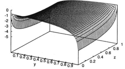
Figure 3: Function g(x, y, z) given by (17) with x = 0.5 .
