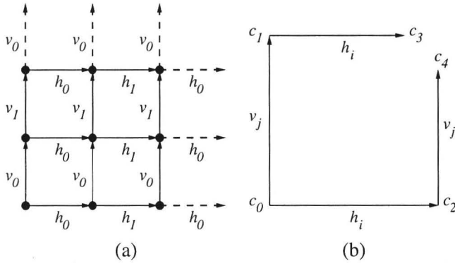
Figure 2: Modeling an even grid \mathcal{G}
