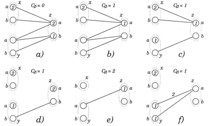
Figure 1: Six equivalent WCSPs (for k = 4 ).
