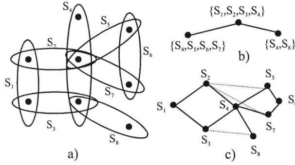
Figure 1: (a) a hypergraph \mathcal{H}' , (b) a hinge decomposition of \mathcal{H}' , and (c) a reduct of dual(\mathcal{H}')
