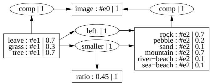
Figure 2: An example (partial) image graph of an input image. Relations are represented as ellipses. Concepts and relation attributes are represented as rectangles.
