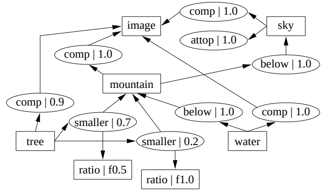
Figure 1: A (partial) model graph representing a mountain-and-lake scene. Relations are represented as ellipses. Concepts and relation attributes are represented as rectangles. Due to space limitation, only some of the concepts, relations, and relation attributes are shown.
