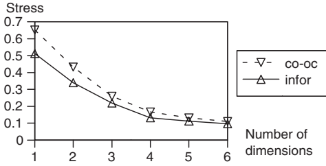
Figure 2: Stress plot of the MDS fitting results. Optimal trade-off between accurate fitting and small number of dimensions is obtained with four dimensions. The space constructed with Donderi's information measurement (infor) has a better fit than that constructed using co-occurrence (co-oc).
