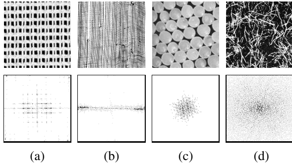
Figure 1: Four types of DFT patterns (bottom) and the corresponding representative textures (top): (a) structured, (b) directional, (c) granular, (d) random.
