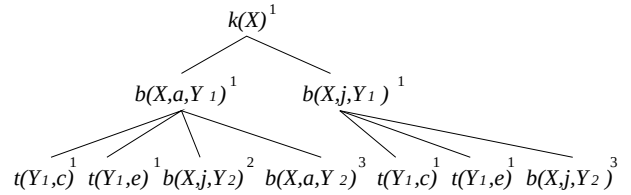
Figure 2: A trie in FARMER
