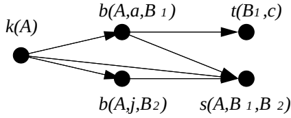
Figure 3: A partial order for a query
