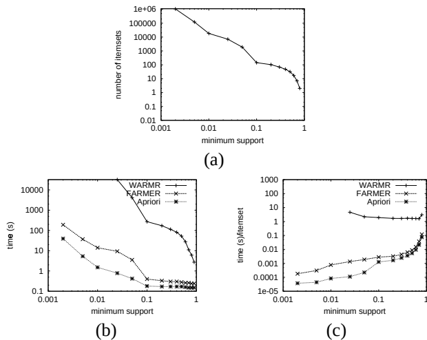
Figure 5: Comparison of results for the digit dataset. (a) The number of frequent itemsets for each minimum support. (b) The execution times of the algorithms. (c) The execution times consumed for each itemset. Note that the scale is logarithmic on both axis.
