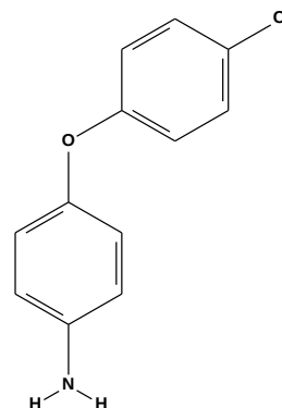
Figure 1: Example compound in a 2-D representation. ' cl-c \sim c \sim c \sim c-o ' is an example fragment occurring in the molecule.
