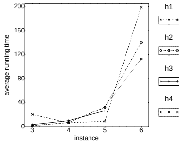
Figure 3: Blockworld problems, average running times
