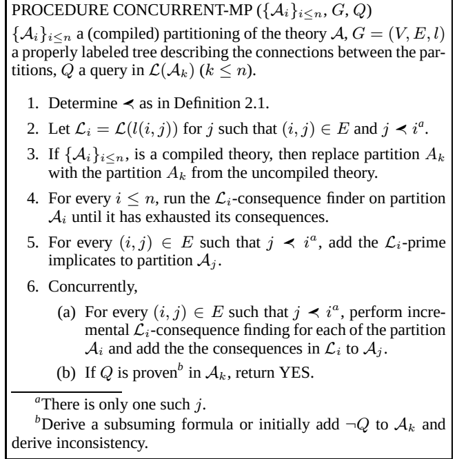
Figure 10: A concurrent message-passing algorithm.
