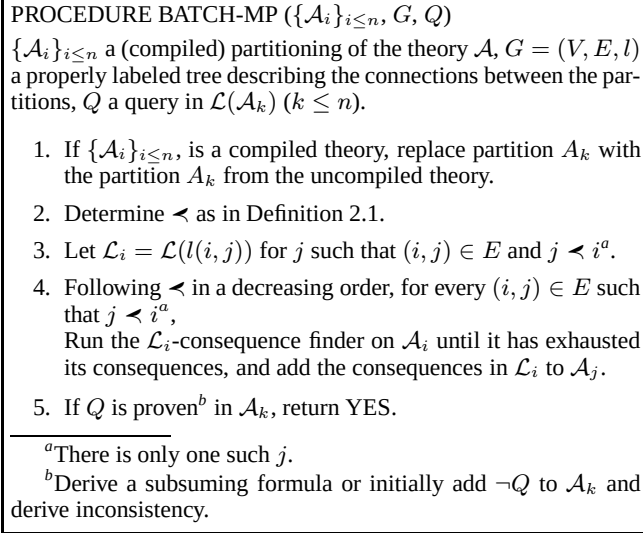
Figure 9: A batch-style message-passing algorithm.
