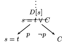
Figure 1: A derivation with splitting and unit resolution
