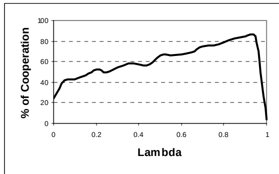
Figure 8: Percentage of trials out of 1,000 that converged to mutual cooperation as a function of the update rate, \lambda . Parameters other than \lambda were selected randomly as described in Table 1.
