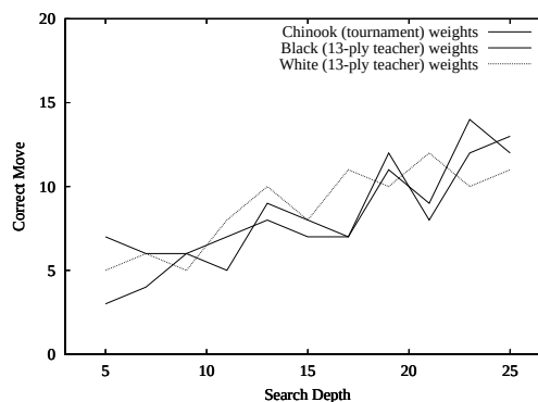
Figure 3: Chinook test set data.
