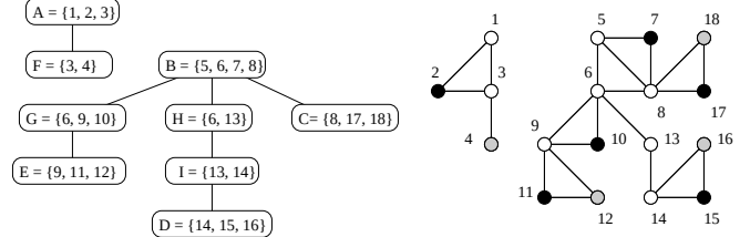
Figure 2: A BCC(DFS, BFS) ordering.
