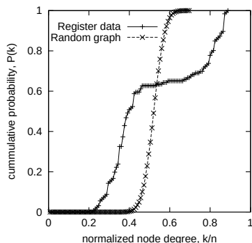
Figure 2: Cumulative probability (y-axis) against the normalized node degree (x-axis). “Register data” is the ze-ro-nin.i.1 register allocation problem which is converted into a graph coloring problem with 125 nodes and 4100 edges. “Random graph” is a random graph of the same size and edge density. Other problems in the DIMACS graph coloring benchmark gave similar results.
