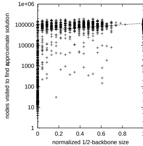
Figure 9: Cost of finding approximate solution within factor 2 of optimal (y-axis, logscale) against normalized 1/2-backbone size (x-axis) for the n = 24 number partitioning problems from Figure 5. The straight line gives the least squares fit to those problems whose backbone is neither complete nor empty.
