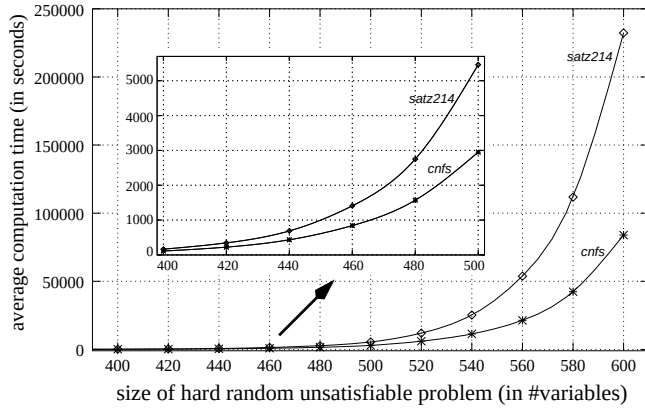
Figure 3: mean computation time of sat214 & cnfs on 3-SAT hard random unsatisfiable formulae from 400 to 600 variables (the same way as for the Figure 2) of sat214 and cnfs for the unsatisfiable formulae within the solved samples. Indeed, the most significant performance figure for a complete algorithm is on unsatisfiable formulae. The gain previously observed between 200 and 400 variables is seen further to increase from 400 to 600. cnfs is 1.85 times faster than sat214 for 500 variables, and 2.78 times faster for 600.
