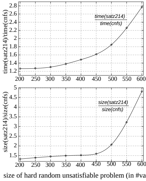
Figure 4: progression of \frac{\text{time}(\text{satz214})}{\text{time}(\text{cnf})} and \frac{\text{size}(\text{satz214})}{\text{size}(\text{cnf})} on unsatisfiable formulae from 200 to 600 variables
