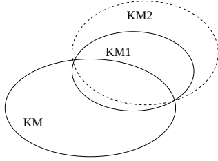
Figure 3: M_1 \leq_M M_2 under the condition w_1 = w_2 , W \not\subset W_1 and W_1 \not\subset W : (b) and (c) hold.
