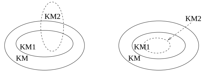
Figure 1: M_1 \leq_M M_2 under the condition w_1 = w_2 and W \subseteq W_1 : (a) or (b) holds.
