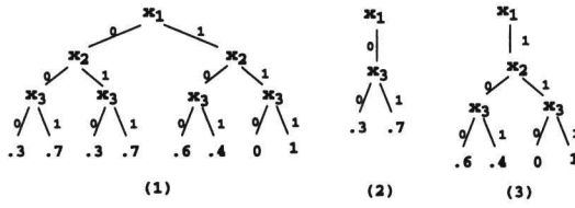
Figure 2: P(x_3|x_1, x_2) and its decomposition.
