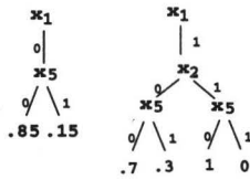
Figure 5: Elimination of variable x_3 .
