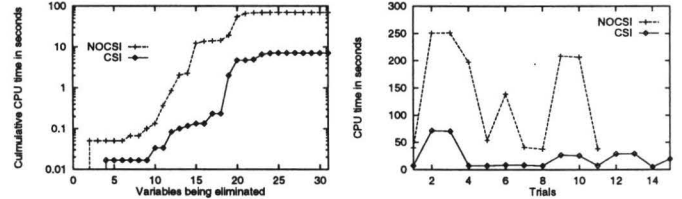
Figure 7: Performances of VE with and without CSI.
