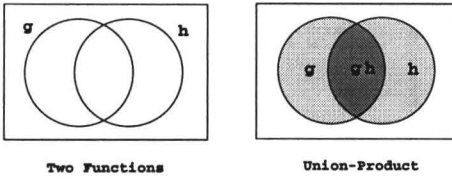
Figure 4: Union-product: The two circles in the left figure represent the domains of two functions g and h . The domain of the union-product g \bowtie h is the union of those of g and h . The union-product equals the product of g and h in the area where both g and h are defined; it equals g in the area where only g is defined; and it equals h in the area where only h is defined.
