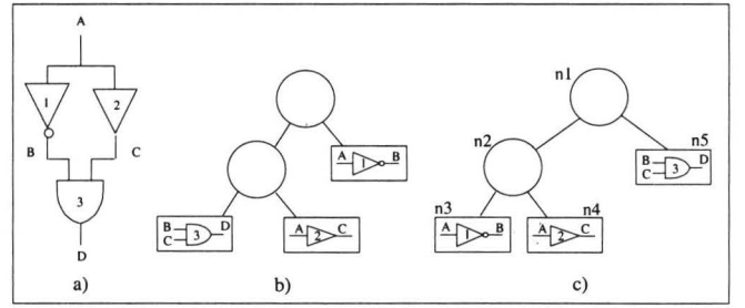
Figure 2: A device with two decomposition trees.
