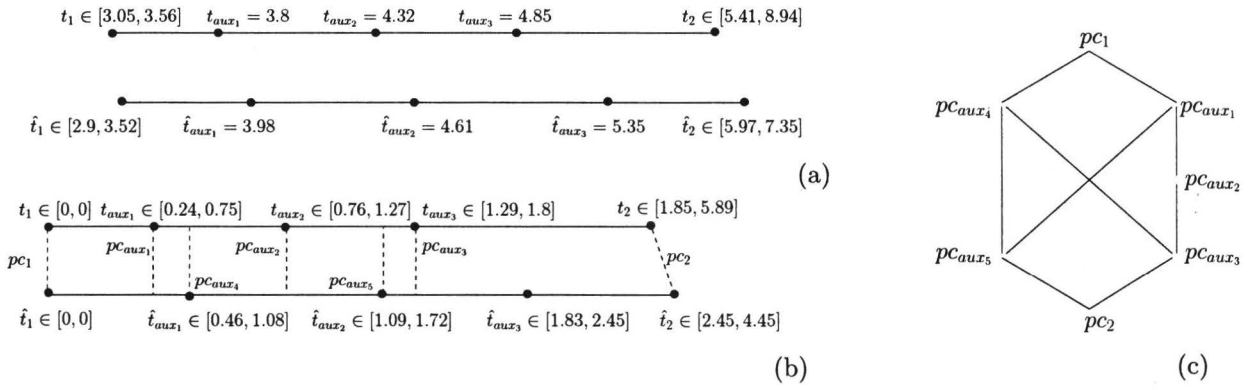
Figure 3: (a) Behavior fragments [t_1, t_2] and [\hat{t}_1, \hat{t}_2] of the behaviors in fig. 1. (b) The synchronized behavior fragments with the auxiliary pairs of comparison and (c) the ordered (top to bottom) auxiliary pairs of comparison.
