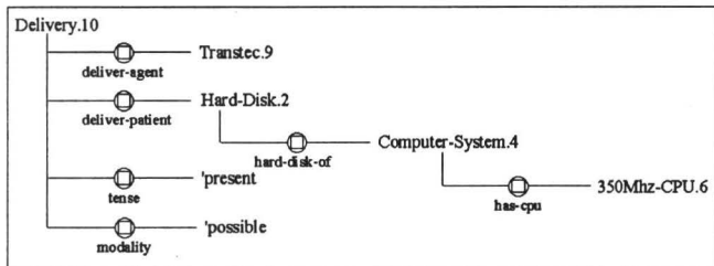
Figure 2: The Corresponding Concept Graph
