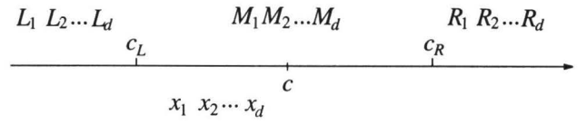
Figure 4: The random cut c and random class distribution x_1, \dots, x_d induced by c
