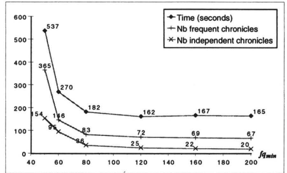
Figure 11: Experiment with ATM network data.
