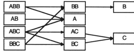
Figure 10: Dependency graph of the frequent chronicles.
