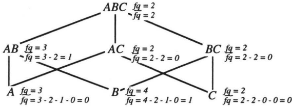
Figure 9: Calculation of \widetilde{fq}(C \sqsubseteq ABC) (with fq_{min}=2 ).
