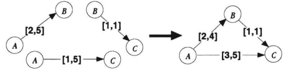
Figure 8: Establishing time constraints.
