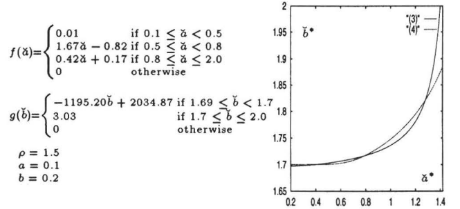
Figure 1: Example with 3 Nash equilibria for SIMUDBP.
