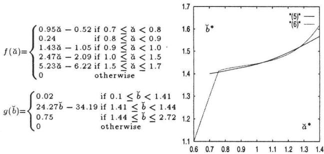
Figure 2: Example with 3 local optima.
