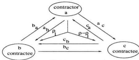
Figure 3: 3-agent contract
