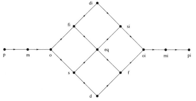
Figure 3: The interval lattice (\mathcal{B}_{int}, \leq) .
