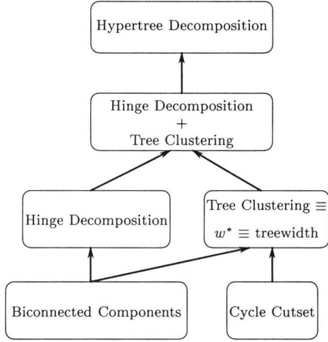
Figure 2: Constraint Tractability Hierarchy
