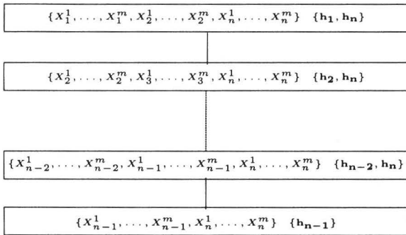
Figure 3: 2-width hypertree decomposition of Circle(n, m)
