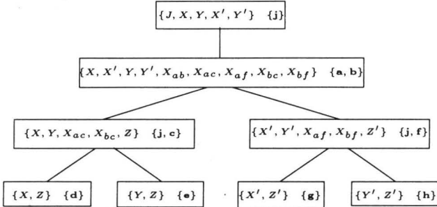
Figure 1: A 2-width hypertree decomposition of \mathcal{H}_1
