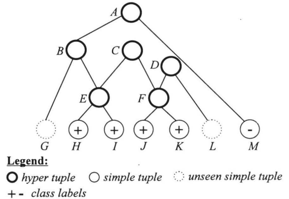
Figure 1: A running example.
