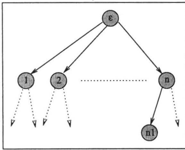
Figure 1: The structure of views
