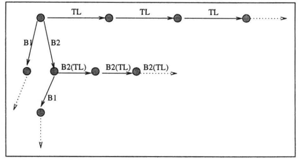
Figure 3: Typical Model Exploration
