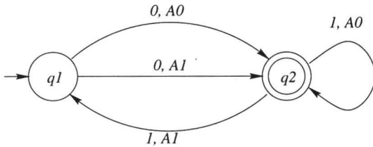
Figure 2: A graphical representation of a Büchi tree automaton accepting the tree from Figure 1.
