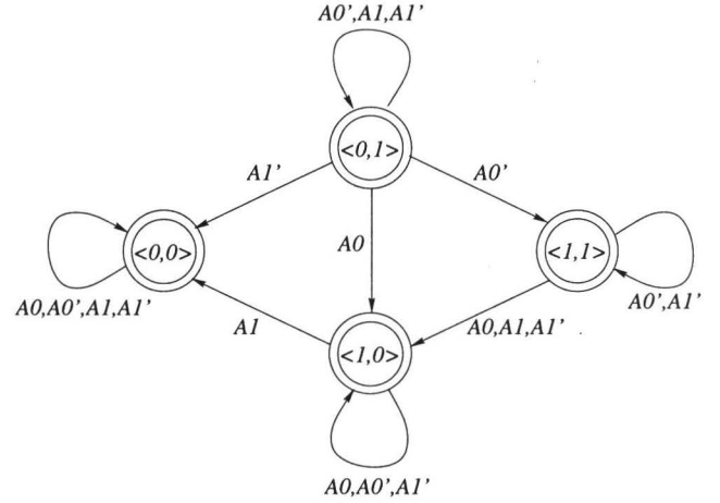
Figure 3: A Büchi tree automaton where the transition function is determined by the successor state axioms from Example 2.
