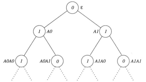
Figure 1: An infinite labeled tree t : \{A_0, A_1\}^* \rightarrow \{0, 1\} with the set of nodes dom(t) = \{A_0, A_1\}^* and labels from \{0, 1\} .
