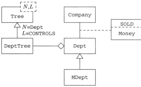
Figure 2: An UML diagram
