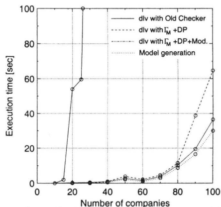
Figure 4: Overall time to compute one stable model
