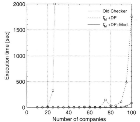
Figure 2: Total model checking time required for the computation of all stable models
