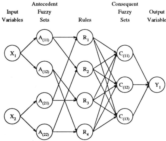
Figure 1: An example of a fuzzy-neural network.
