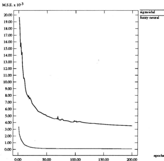
Figure 2: Mean Squared Error (M.S.E.) curves on the training data for the fuzzy-neural network and the sigmoidal neural network, averaged over 10 trials, with 200 epochs in each trial.
