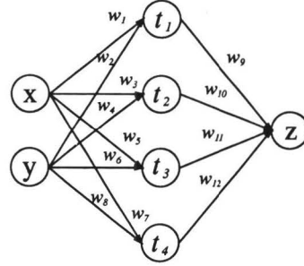
Figure 2: Neural Network
