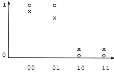
Figure 1: Approximation
