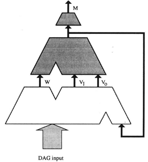
Figure 2: The generalized recurrent network architecture for processing data structures; the processing takes place in the extended time space dimension. The neuron activations are recorded in the lower module, which is also responsible for feeding the layer of neurons, according to the defined topological sorting.
