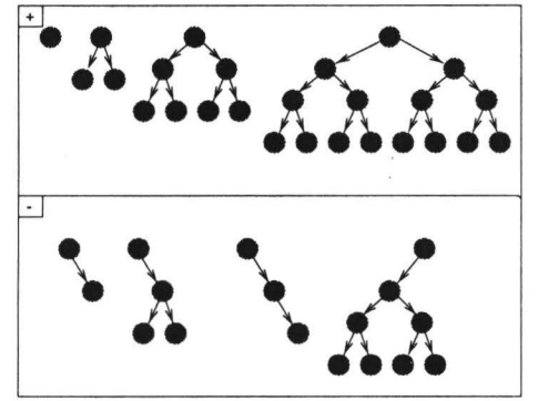
Figure 5: The problem of learning perfect binary trees. The associated error function has no local minima, provided that one uses 8 hidden units.
