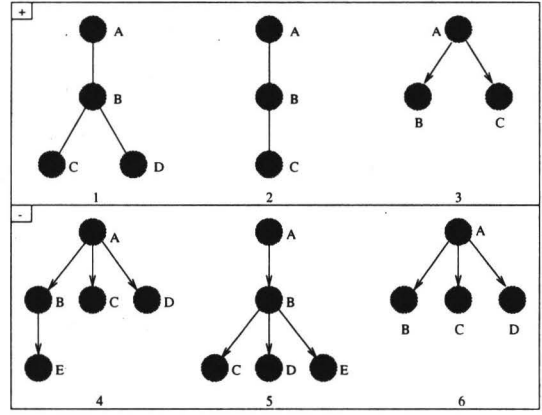
Figure 3: The problem of classifying DOAGs depending the their outdegree. Positive DOAGs are those with outdegree less than three. Since \mathcal{D}_L \uparrow = 8 , a network with 8 hidden units can be used in order to avoid local minima. Note that the letters attached to the nodes are only used as pointers.
