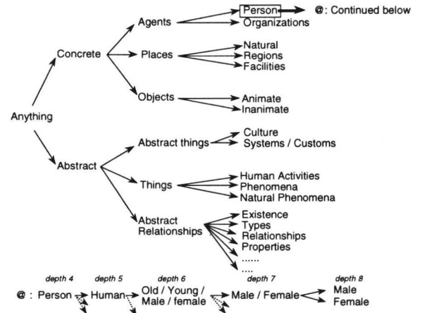
Figure 1: The upper levels of the type hierarchy
