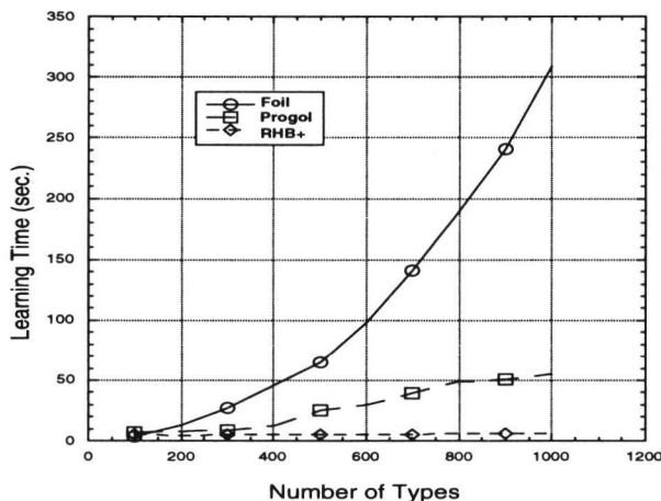
Figure 2: Learning time vs type hierarchy size
