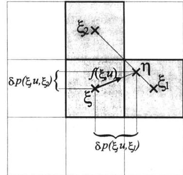
Figure 2: A geometrical interpretation of the FD scheme. The transition probabilities p(\xi, u, \xi_i) of the corresponding MDP are the coordinates of the vector \frac{1}{\delta} \xi \eta with \eta the projection of \xi onto the segment (\xi_1 \xi_2) in a direction parallel to f(\xi, u) .
