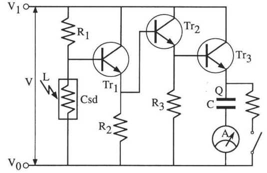
Figure 2: A circuit of photo-meter
