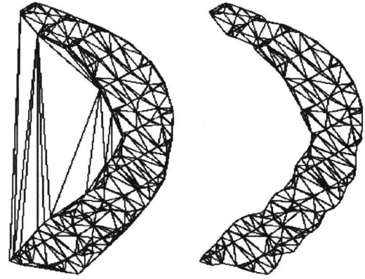
Figure 3: Sculpturing: Recover the shape of the 2D projection of a vortex by removing the exterior triangles from the delaunay triangulation. An exterior triangle is one whose circumcircle is much larger than the triangle (in terms of area). The meridians of the generalized cylinder representation of the vortex are found by backprojecting the boundary of the sculptured triangulation.
