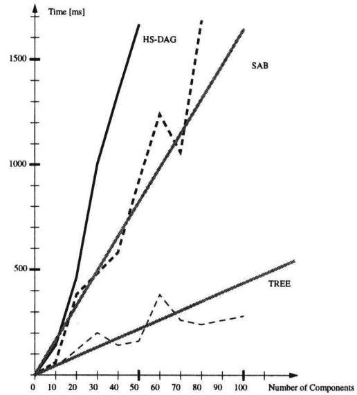
Figure 3: Performance of TREE_DIAG , HS-DAG , and SAB for \frac{|COMP|}{2} inputs
