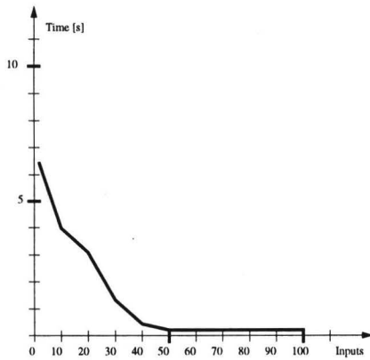
Figure 5: Influence of input number on TREE_DIAG , for |COMPS| = 100
