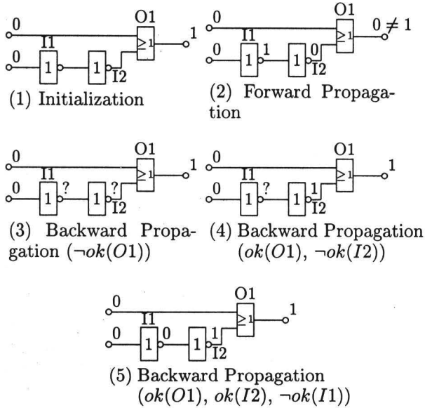
Figure 2: How TREE_DIAG works
