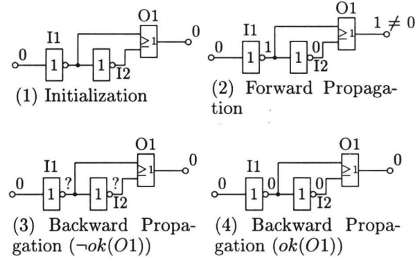
Figure 6: A simple Example explaining DAG_DIAG
