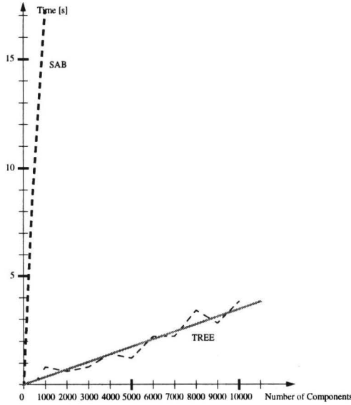
Figure 4: Performance of TREE_DIAG for \frac{|COMPS|}{2} inputs
